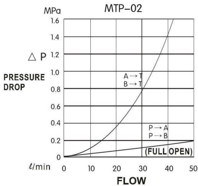
A. PRESSURE DROP-FLOW CHARACTERISTICS:
